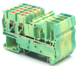
RPV 2.5-TWIN/1P-PE RPV 2.5-QUATTRO/2P-PE
