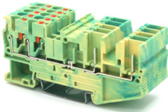
RPV 2.5-TWIN/1P-PE RPV 2.5-QUATTRO/2P-PE
